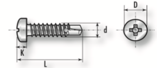
Recessed pan head self-drilling screws
