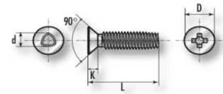
Recessed countersunk (flat) thread rolling screws for ISO metric thread Product grade A
